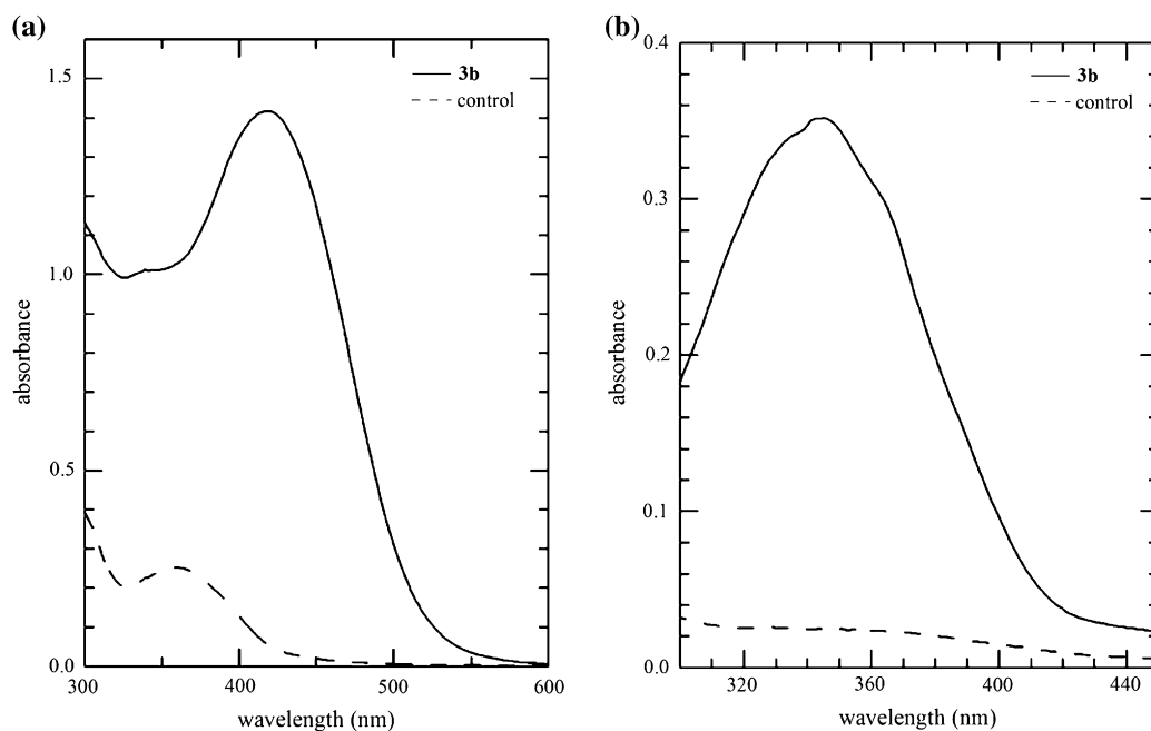
Fig. 5. UV-vis spectra of (a) thymol blue/ 3b system ( [\mathbf{3b}] = 2.19 \times 10^{-6} \text{ mol L}^{-1} ) and (b) alizarin yellow/ 3b system ( [\mathbf{3b}] = 1.07 \times 10^{-6} \text{ mol L}^{-1} ) in \text{CHCl}_3 .
