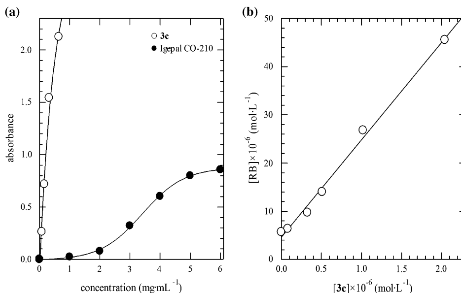
Fig. 6. (a) Absorbance at \lambda_{\max} of RB/3c system (open circle, \lambda_{\max} = 578 nm) and RB/IGP system (closed circle, \lambda_{\max} = 560 nm) in CHCl 3 . (b) Concentration of encapsulated RB, [RB] versus [3c].
