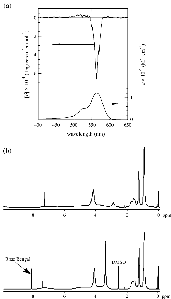
Fig. 4. (a) CD (upper) and UV (lower) spectra of RB/ 3b system in \text{CHCl}_3 using a 5 mm path length (RB in 3b /chloroform = 4.52 \times 10^{-5} \text{ mol L}^{-1} ). (b) ^1\text{H} NMR spectra of RB/ 3b system in \text{CDCl}_3 (upper) and in \text{CDCl}_3/\text{DMSO-}d_6 (3/2, v/v) (lower).
