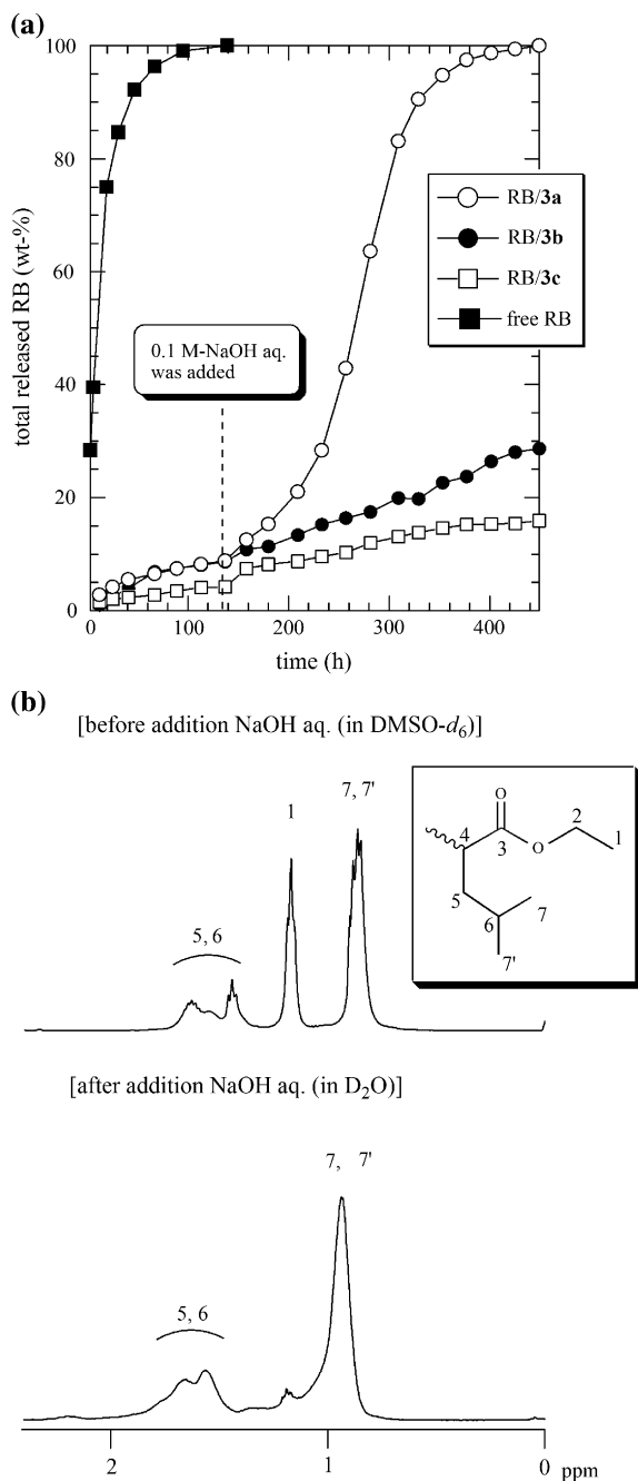
Fig. 7. (a) Release of RB from the RB/3a–c systems in water at 37 °C. (b) 1 H NMR spectra of RB/3a after the beginning of the release experiment for 120 h (before addition of 0.1 mol L -1 aqueous NaOH) (upper) in DMSO- d 6 and 450 h (after addition of 0.1 mol L -1 aqueous NaOH) (lower) in D 2 O.
