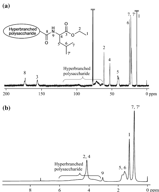
Fig. 1. (a) 13 C NMR and (b) 1 H NMR spectra of 3b in CDCl 3 .
