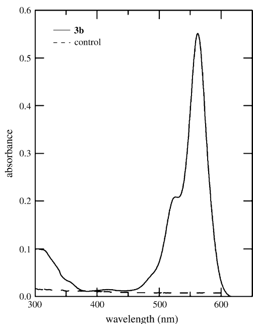
Fig. 3. UV–vis spectra of RB/ 3b system ( [3b] = 2.45 \times 10^{-7} \text{ mol L}^{-1} ) in \text{CHCl}_3 .
